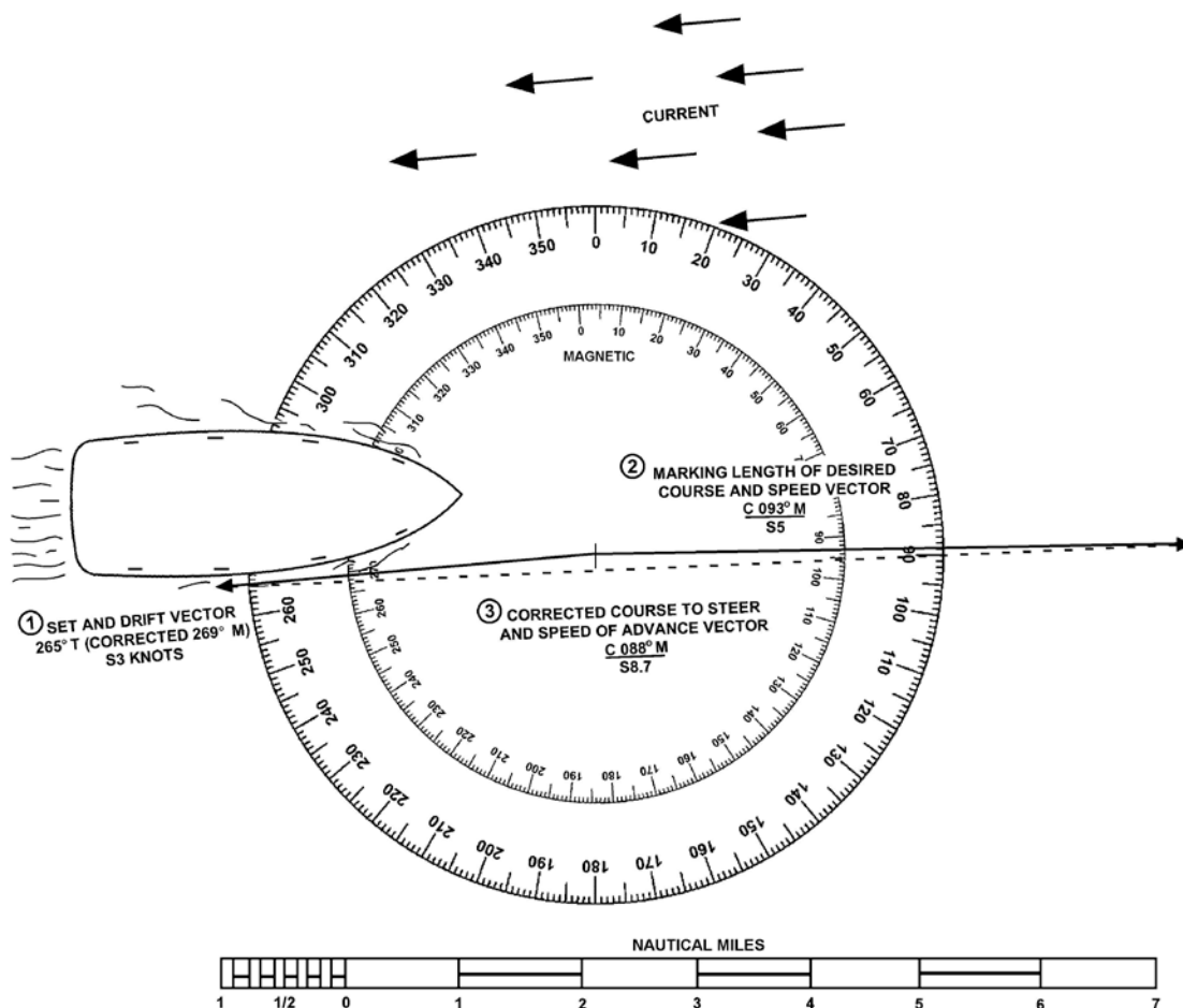
Figure 3-82 Plotting Set and Drift to Determine Course to Steer
