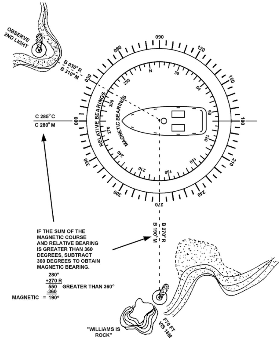
Figure 3-48 Converting Relative Bearings to Magnetic; Sums Greater than 360°
