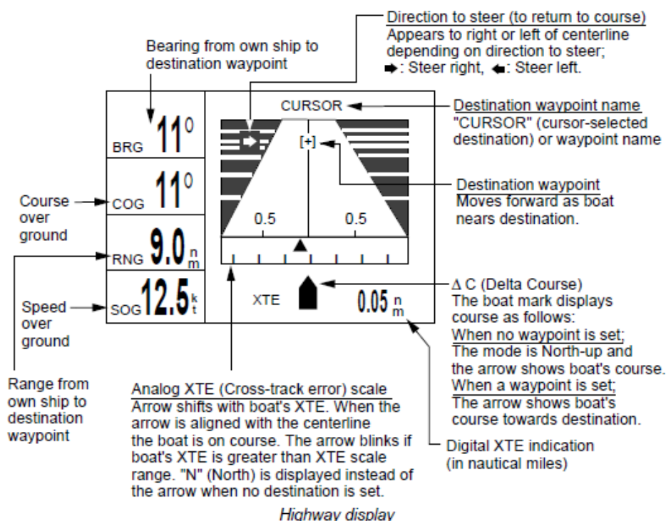
Figure 3-76 GPS Highway Display
