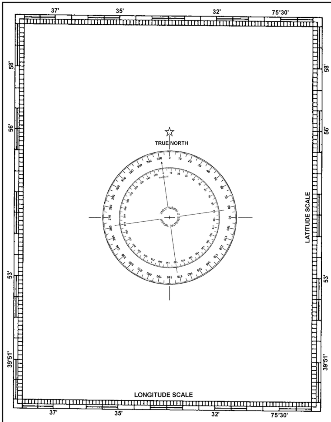
Figure 3-7 Chart Orientation
