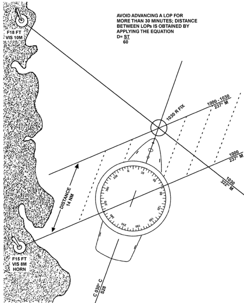
Figure 3-80 Running Fix
