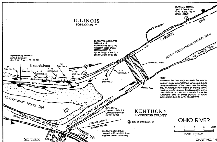
Figure 3-84 Sample River Chart
