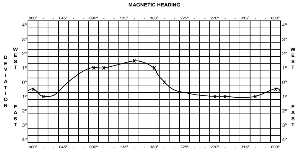
Figure 3-44 Example Deviation Curve
