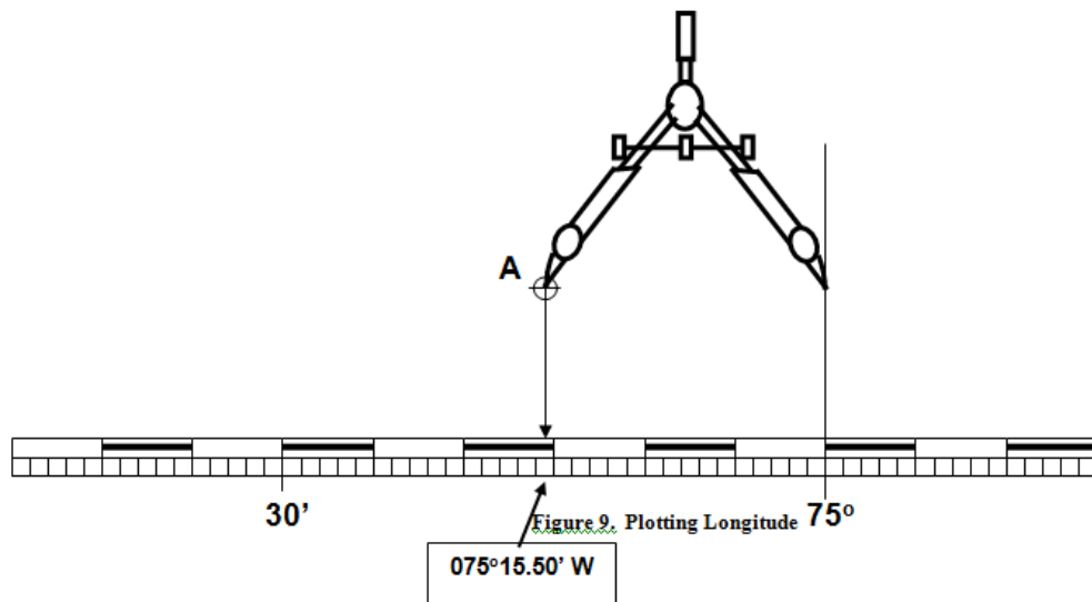
Figure 3-52 Finding the Longitude of a Position
