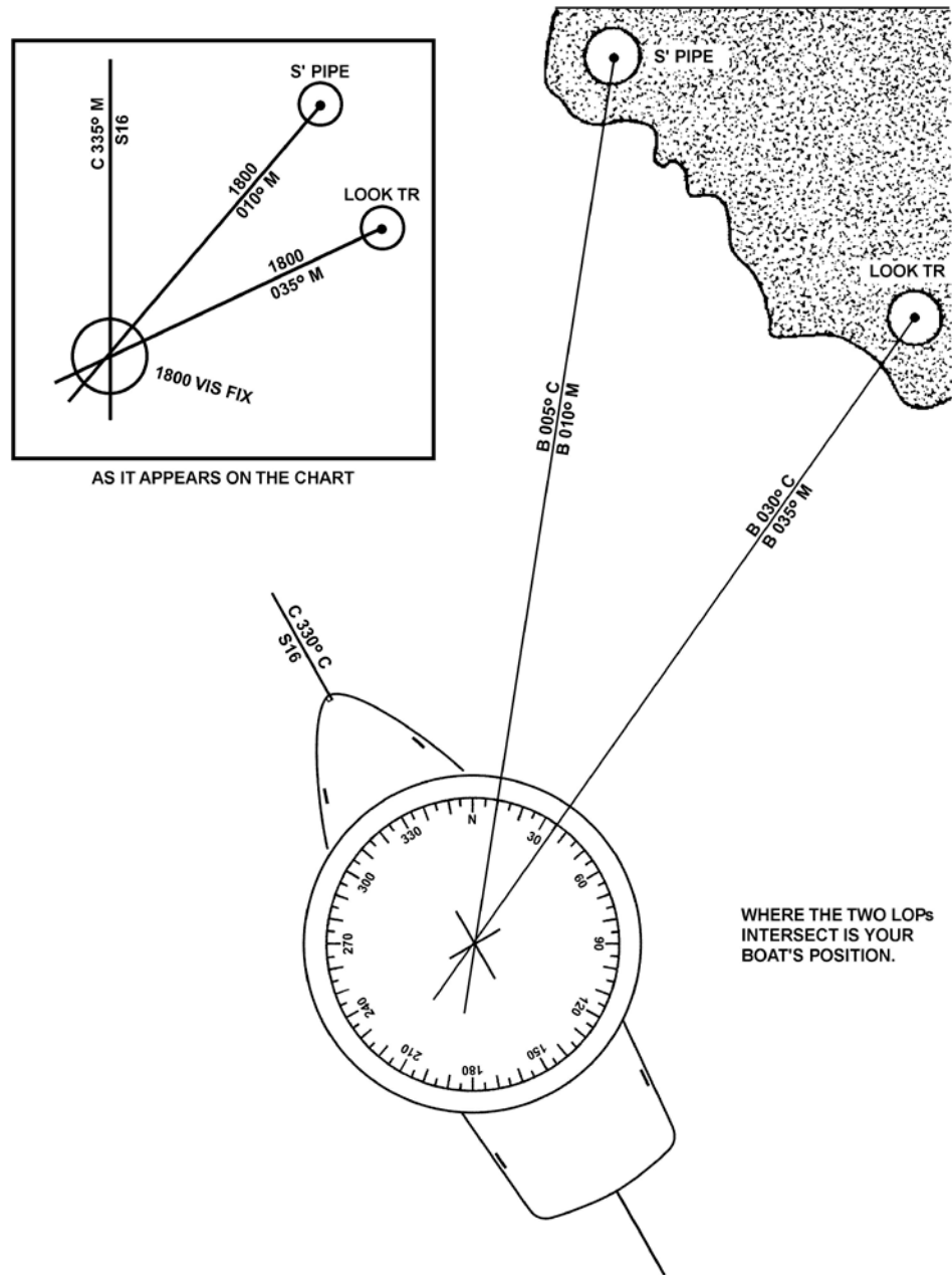
Figure 3-63 Fix Using Visual Bearings
