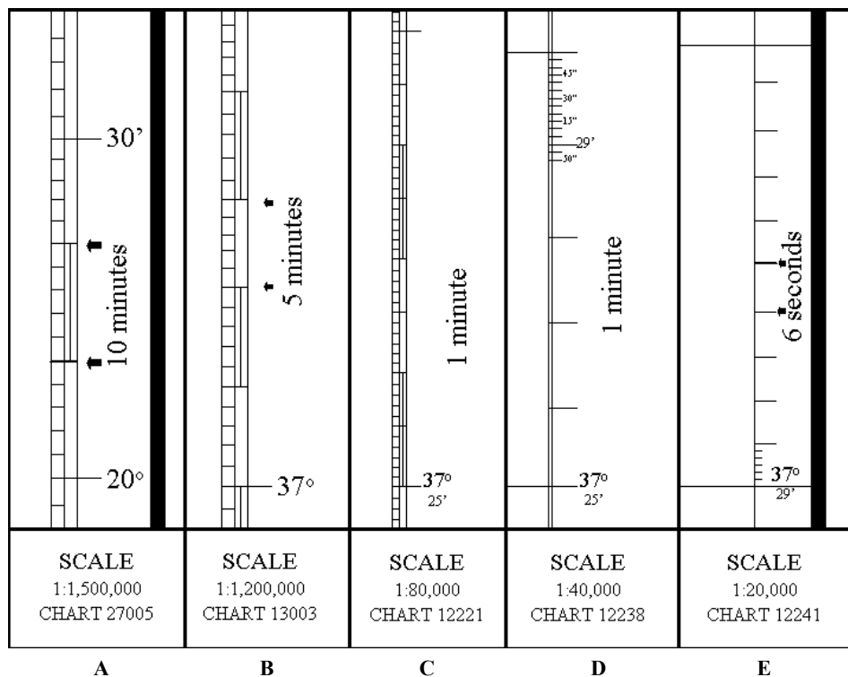
Figure 3-53 Chart Scales
