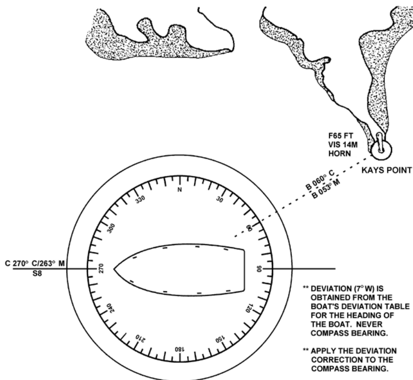
Figure 3-47 Converting Compass Bearing to Magnetic
