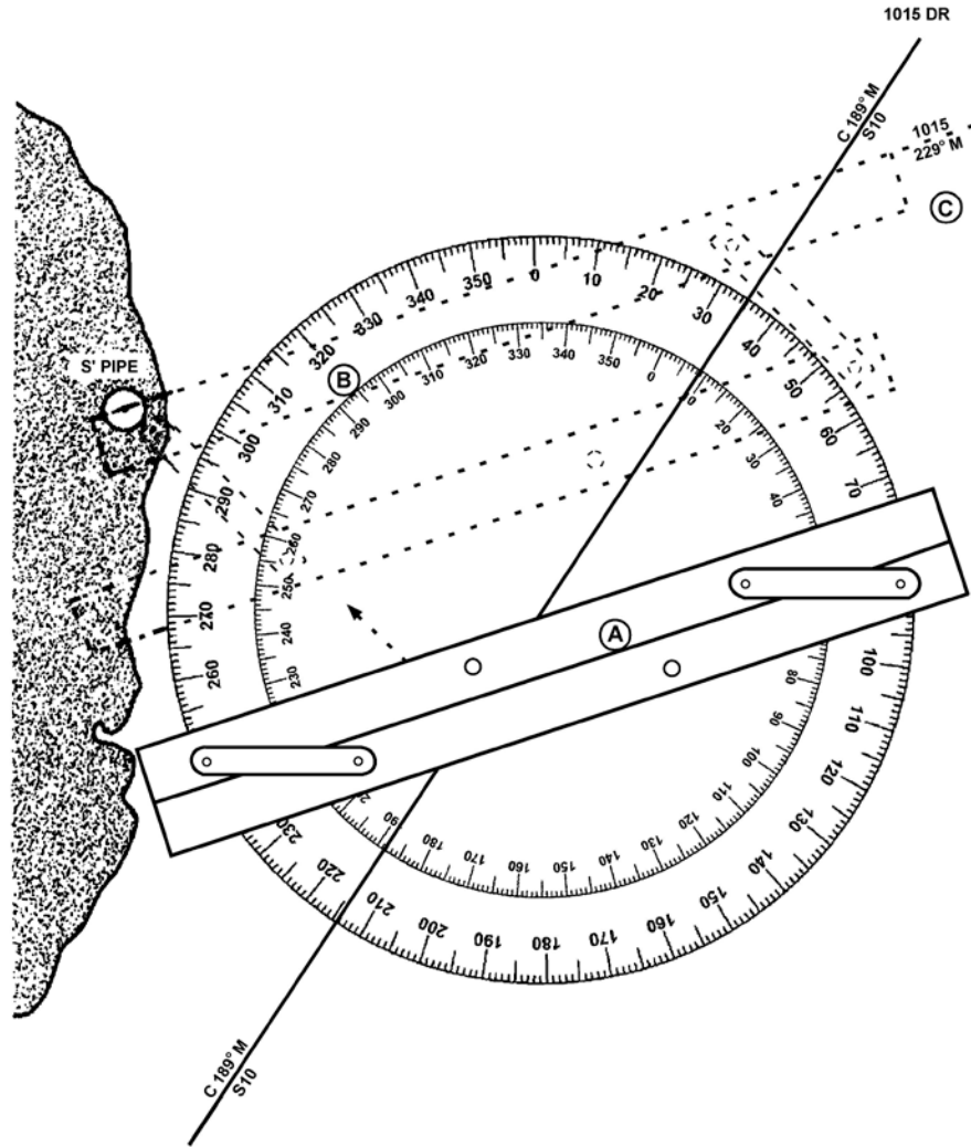
Figure 3-60 Plotting LOP
