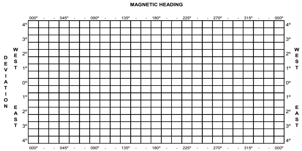
Figure 3-43 Deviation Curve
