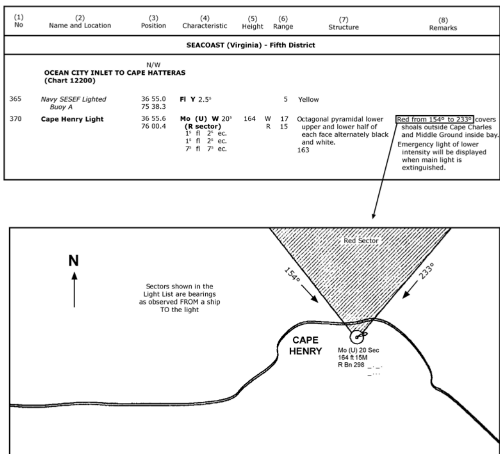
Figure 2-7 Sector Light
