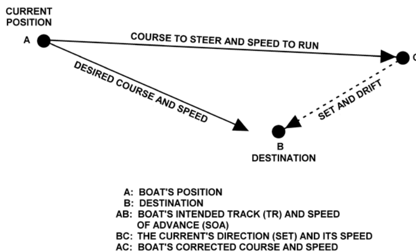
Figure 3-81 Current Triangle
