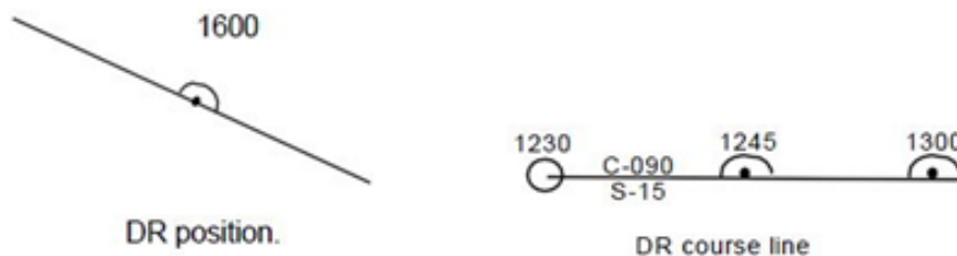
Figure 3-77 Labelling a DR Position & Course
