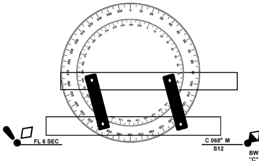
Figure 3-69 Laying Trackline
