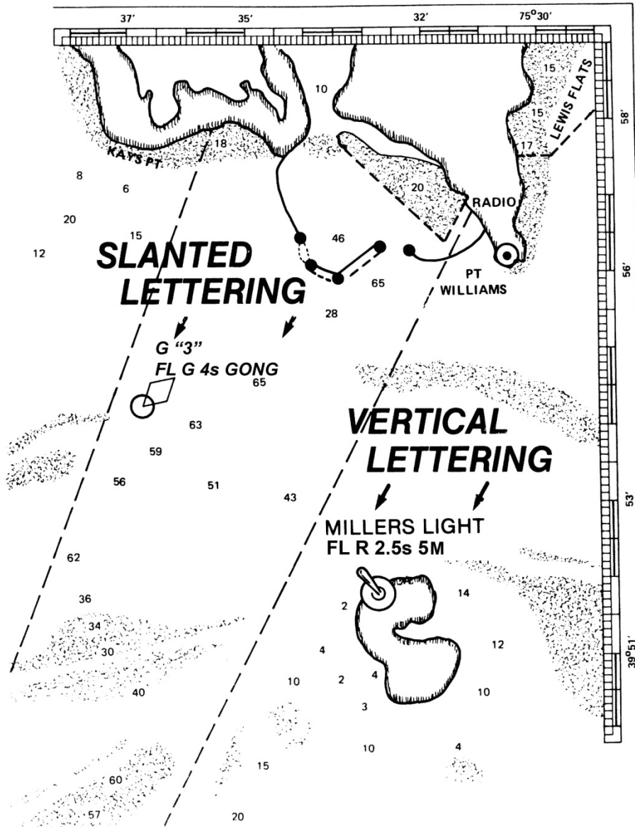
Figure 3-9 Chart Lettering
