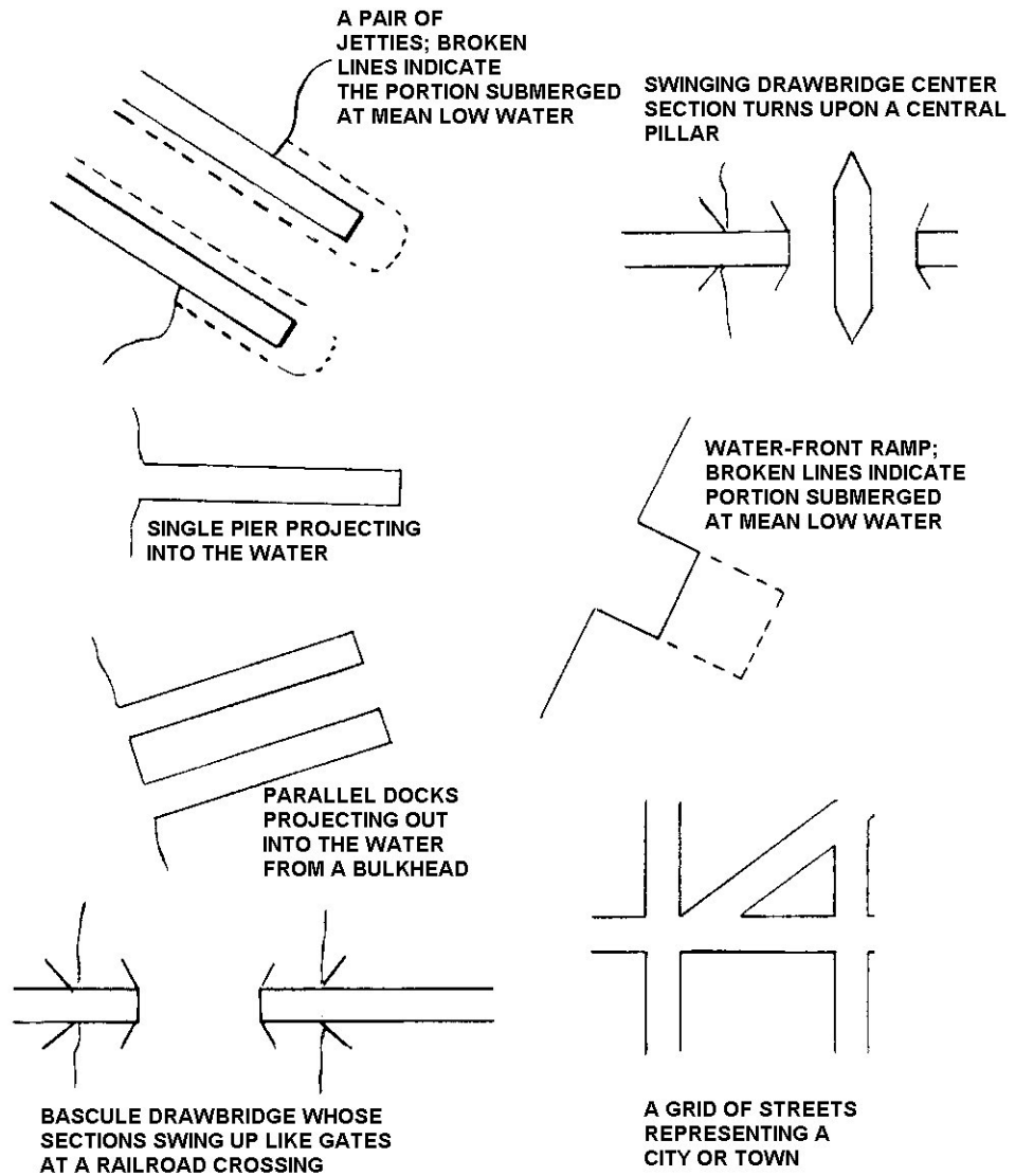
Figure 3-12 Structures
