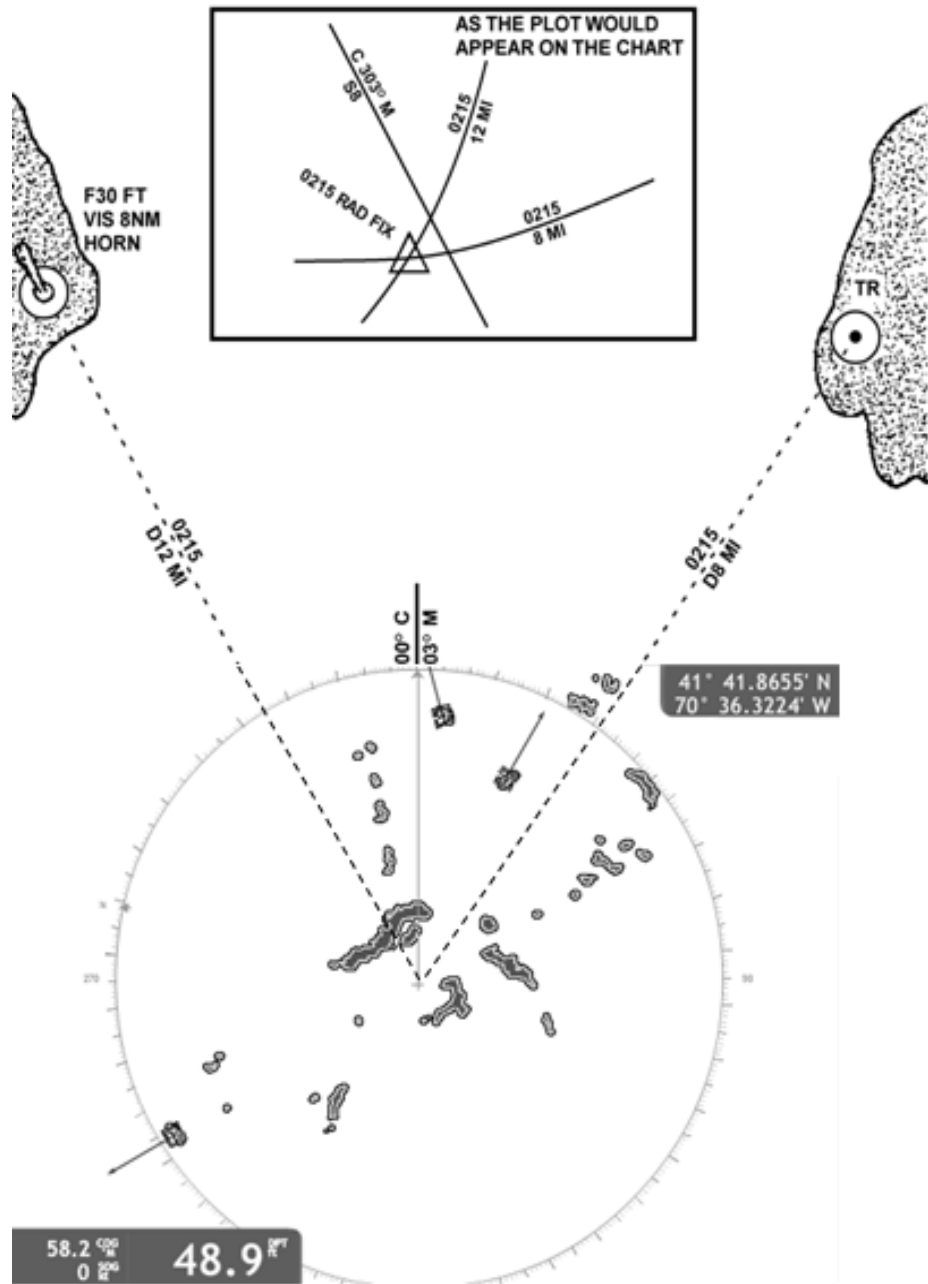
Figure 3-61 Obtaining a Radar Fix Using VRM
