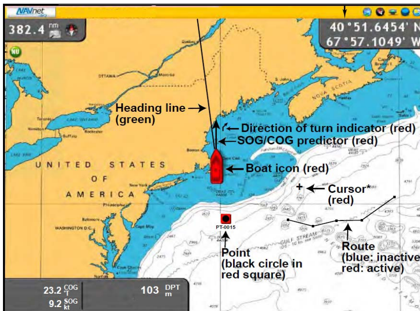
Figure 3-19 Boat Position Symbol
