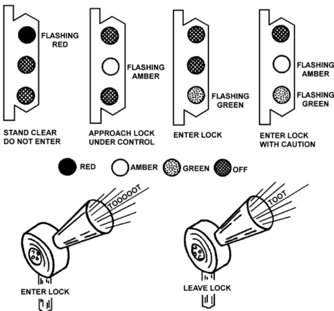
Figure 3-86 Standard Locking Signals
