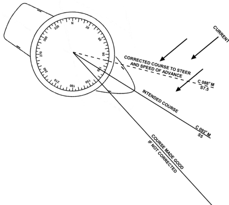
Figure 3-83 Compensating for Set and Drift
