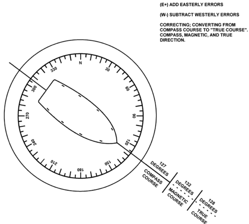
Figure 3-45 Applying Compass Error, Correcting
