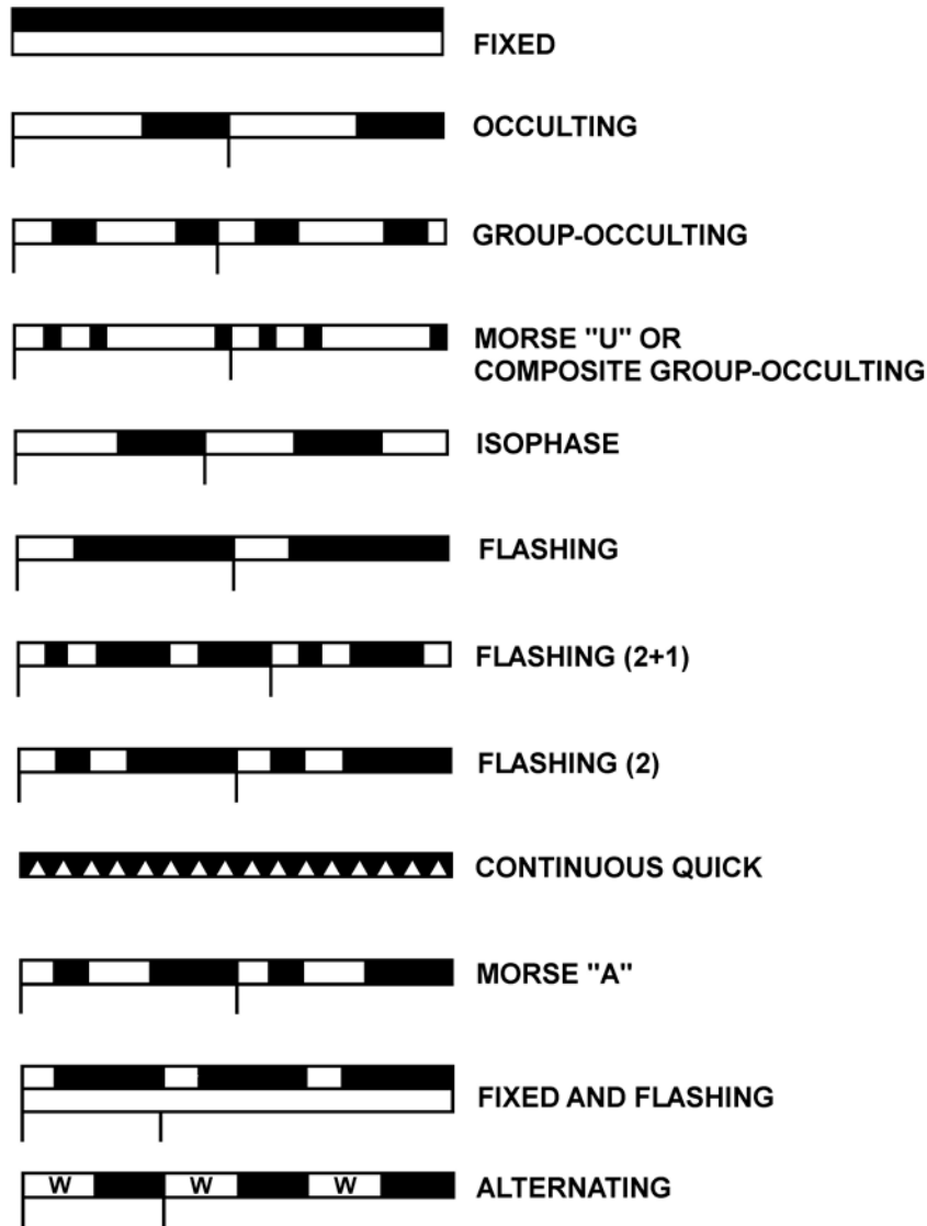
Figure 2-4 Light Characteristics
