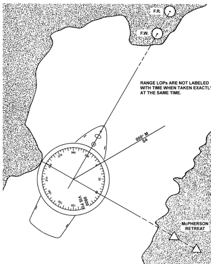
Figure 3-64 Visual Fix Using Terrestrial Ranges
