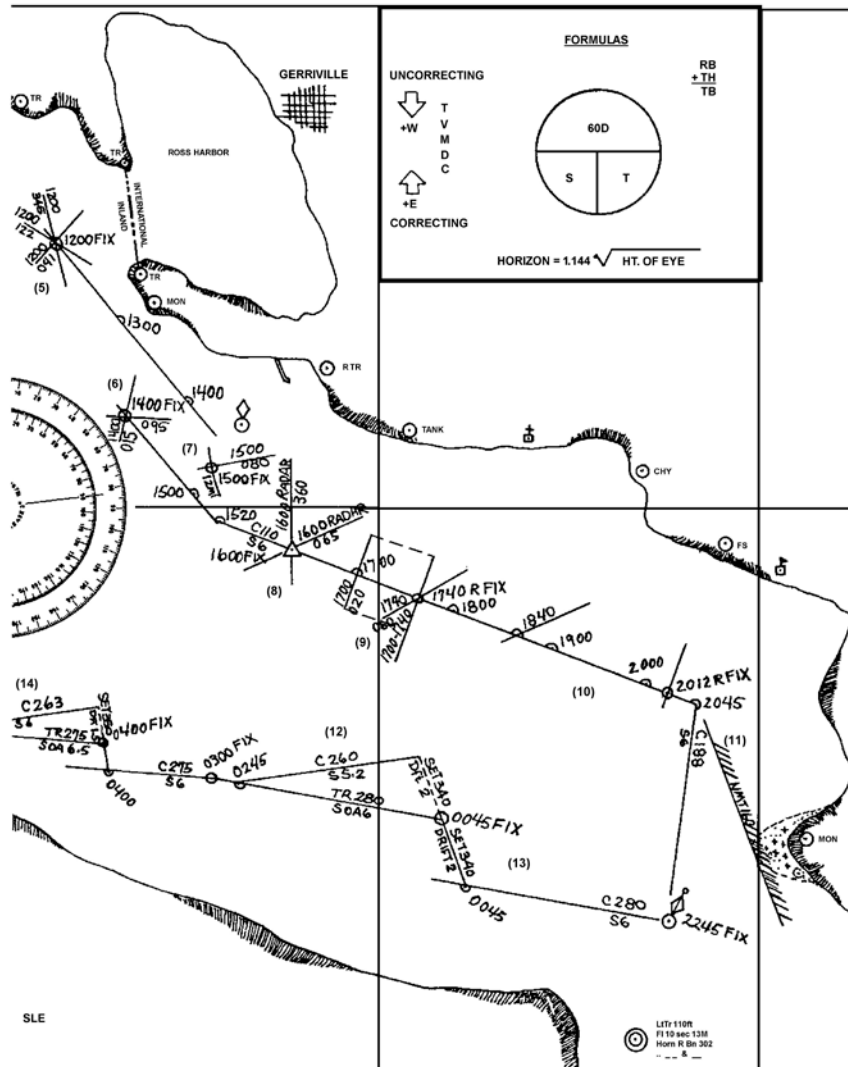
Figure 3-79 Sample DR Plot
