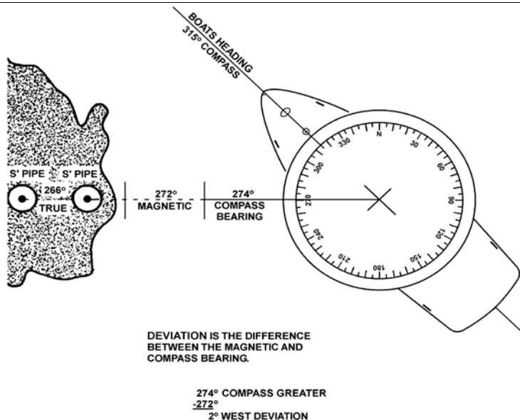
Figure 3-42 Deviation Check Using Ranges
