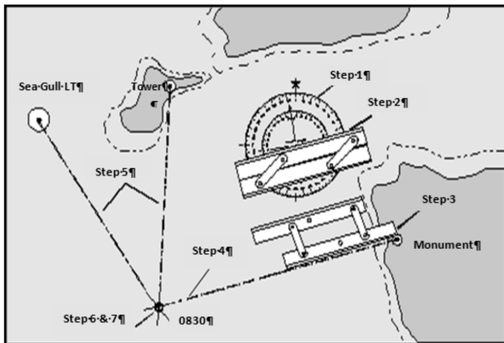
Figure 3-62 Obtaining Radar Fix Using EBL
