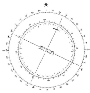
Figure 3-40 Easterly Error Variation
