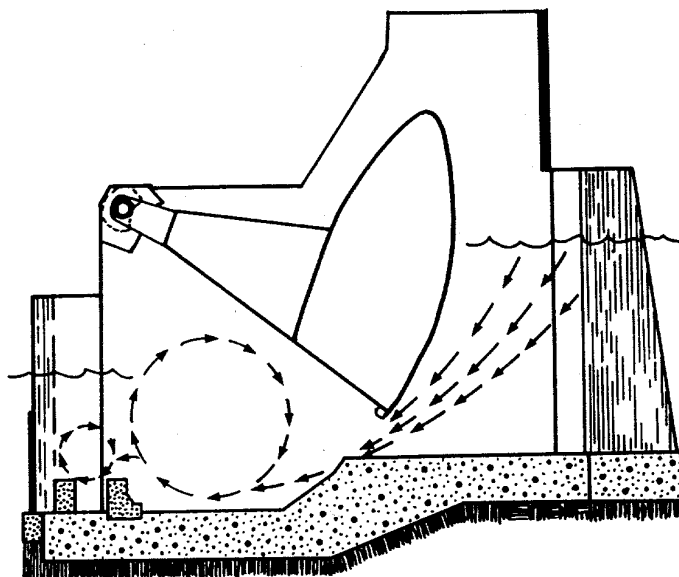
Figure 3-85 Roller Gate Dam
